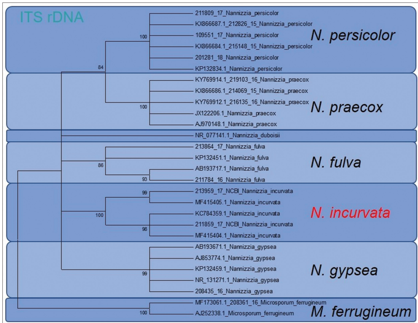
Figure 3a: Phylogenetic analysis of both from the here reported patients isolated Nannizzia incurvata strains. Based on ITS region of the rDNA, the dendrogram showed clear genetic differentiation between Nannizzia incurvata and the close related species Nannizzia gypsea and Nannizzia fulva
